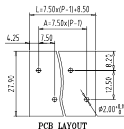
PCB LAYOUT
